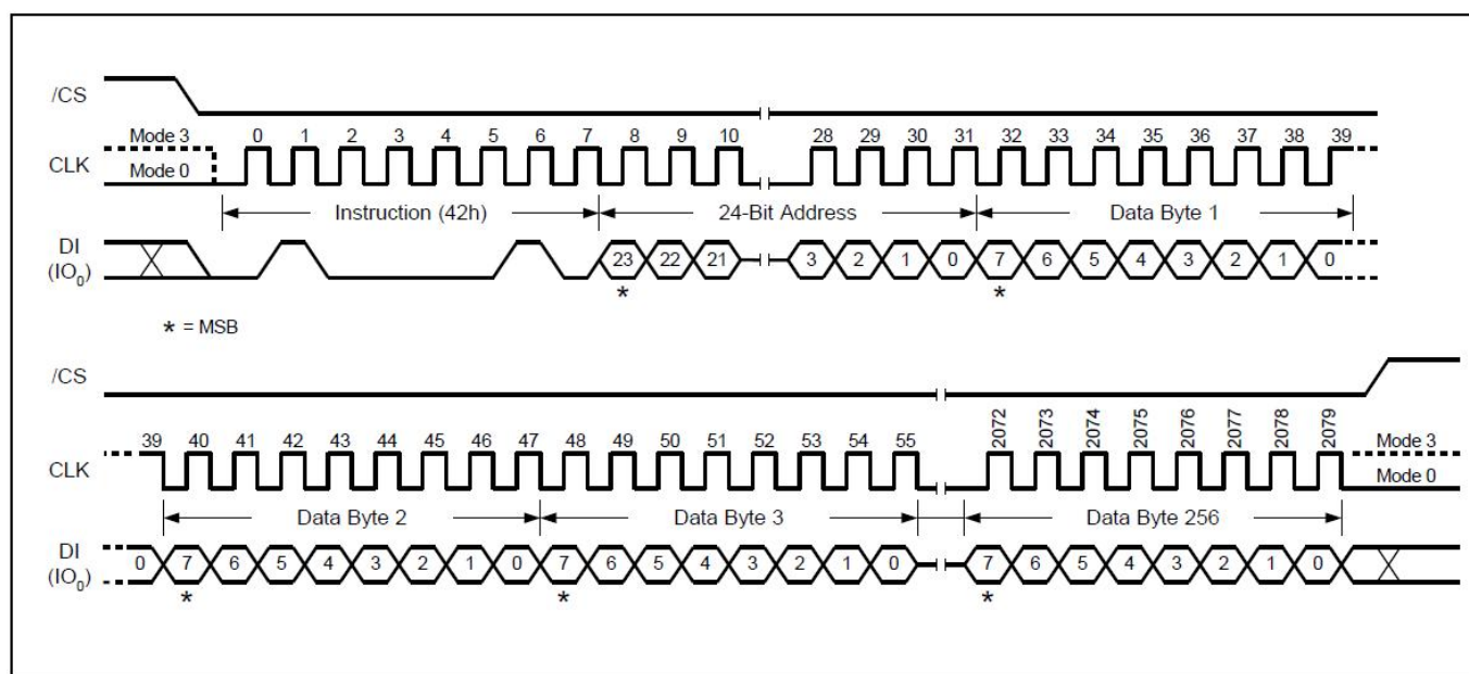
Figure 34. Program Security Registers Instruction (SPI Mode only)
